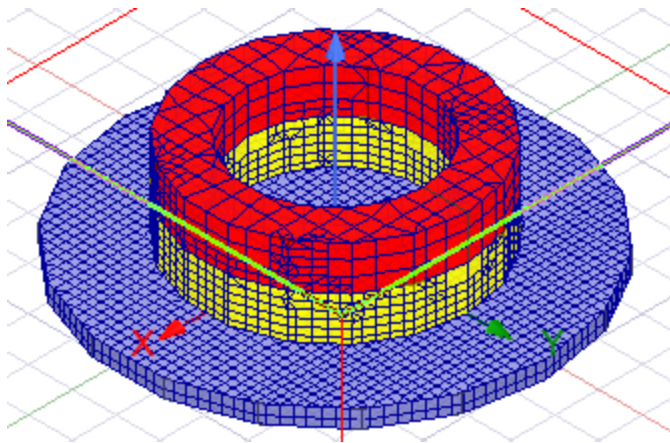
Figure 3-18: Global Mesh
