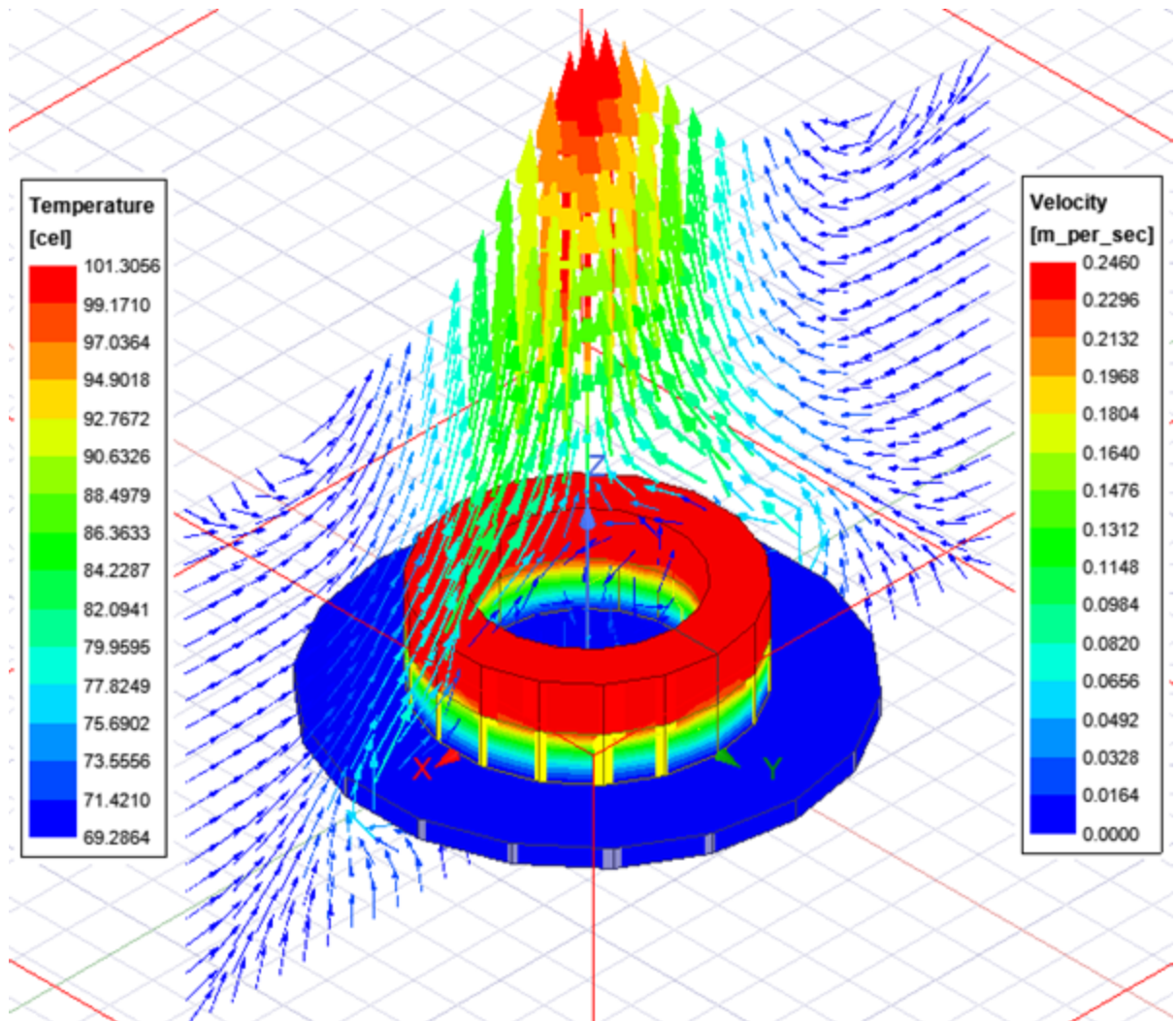
Figure 4-3: Velocity vectors on a plane
